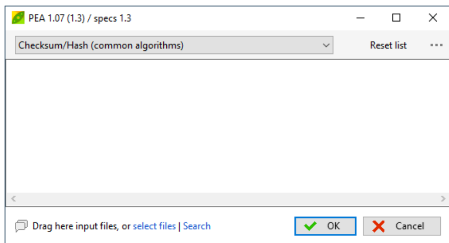
Image 29: PeaUtils
