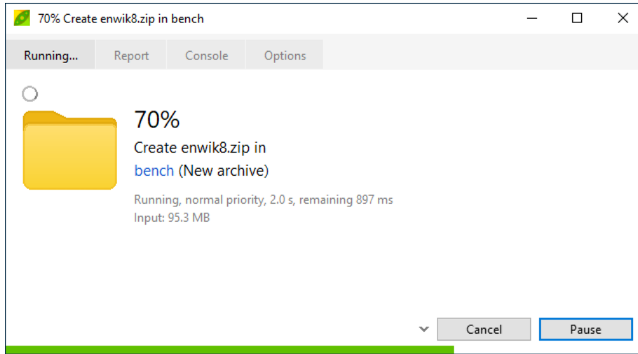
Image 27: PeaLauncher instance
