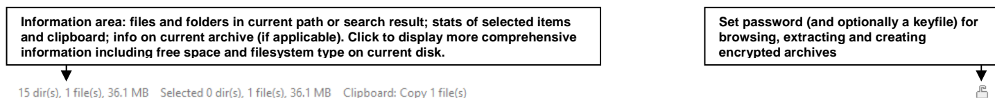
Image 14: status bar
