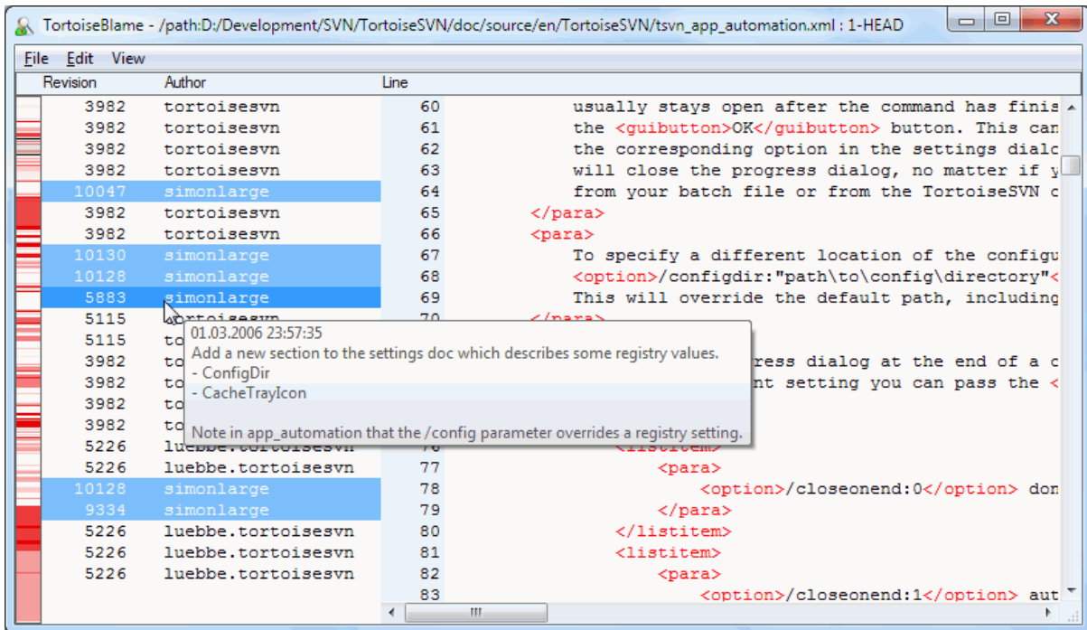
Figure 4.59. TortoiseBlame
